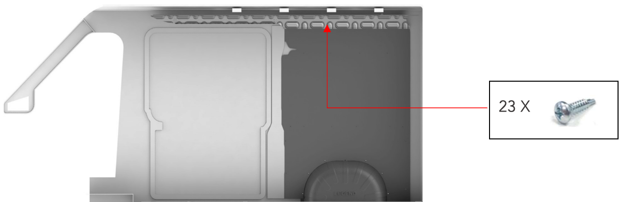
Figure 24 "Passenger side Top Sills installed"
