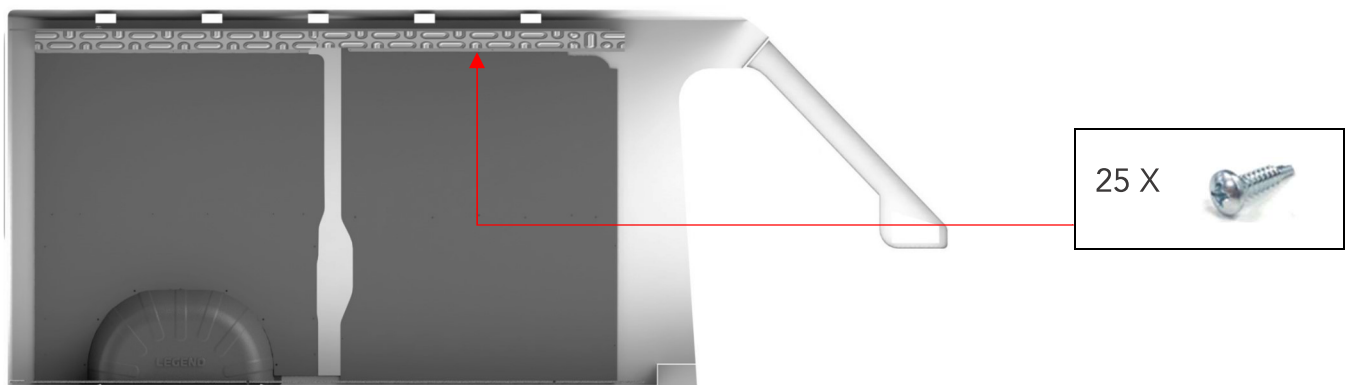
Figure 18 "Driver side Top Sills installed"
