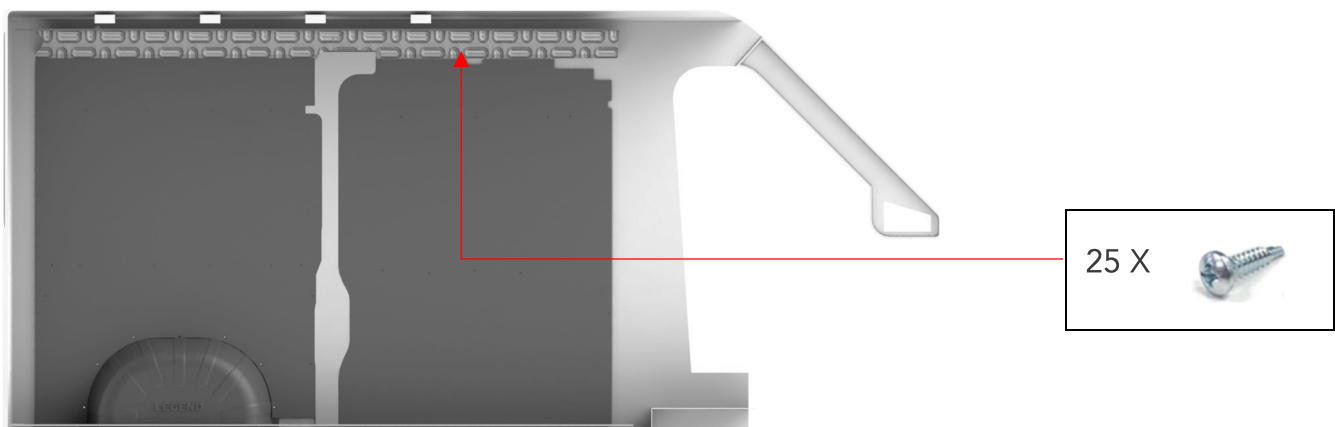
Figure 22 "Driver side Top Sills installed"
