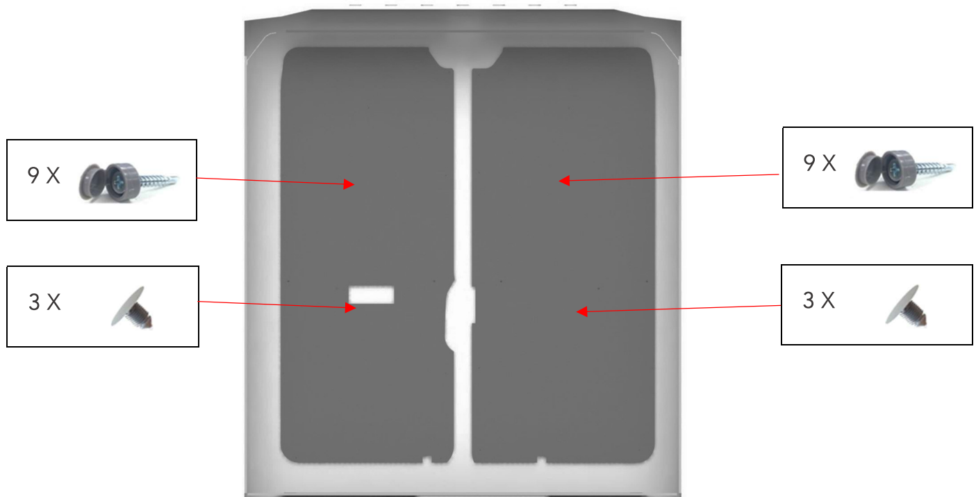
Figure 27 "Rear Door Liners Installed"
