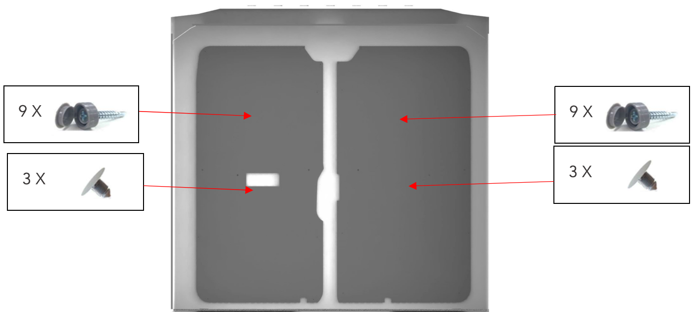
Figure 25 "Rear Door Liners Installed"
