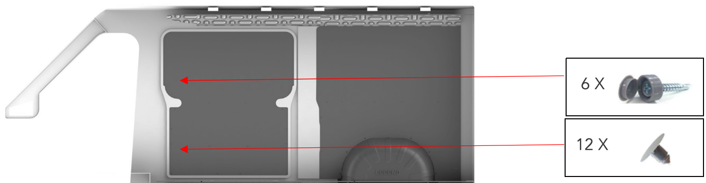
Figure 26 "Passenger Side Sliding Door Liner Installed"
