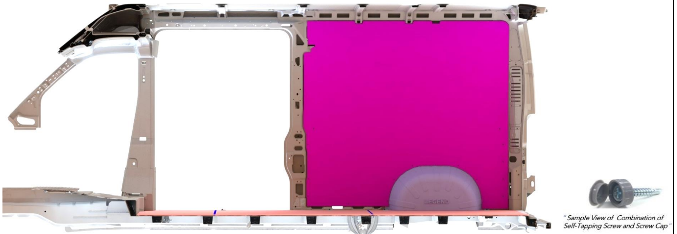
" Passenger Side Wall Liner Installed" This is view from Inside of the Van- Viewing from Driver Side
