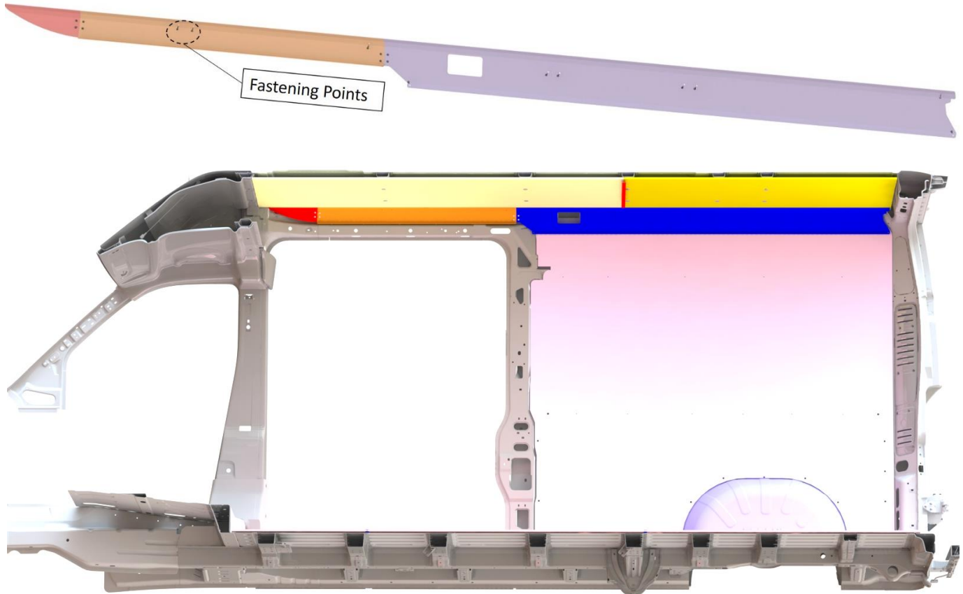
"Passenger Side Top Sills Installed" This is view from inside the vehicle when Viewing from Passenger Side
