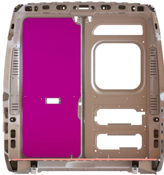
"Passenger Side Rear Door Liner Installed" This is view from Inside of the Van- Viewing from Front towards Rear Doors
