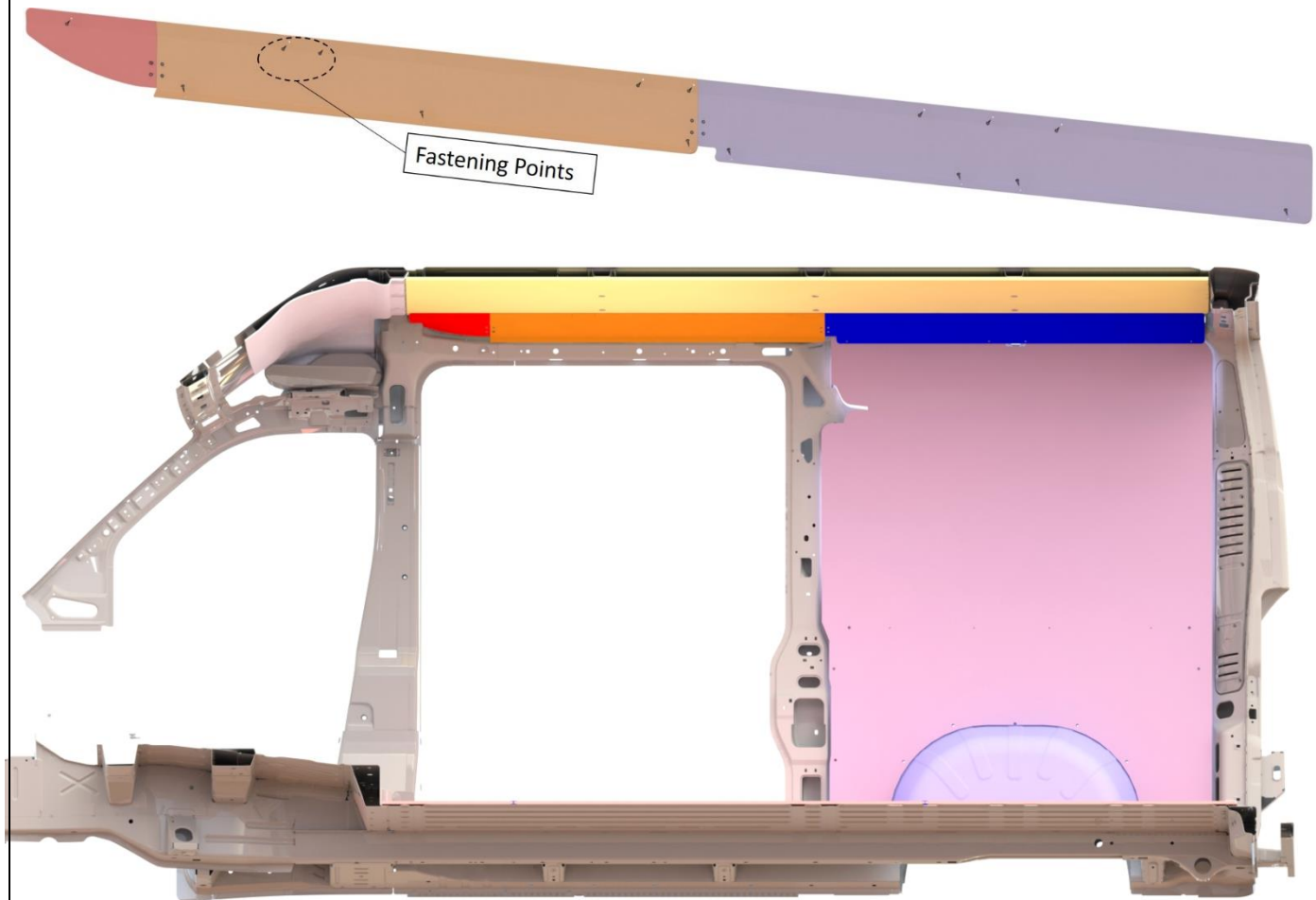
"Passenger Side Top Sills Installed" This is view from inside the vehicle when Viewing from Passenger Side
