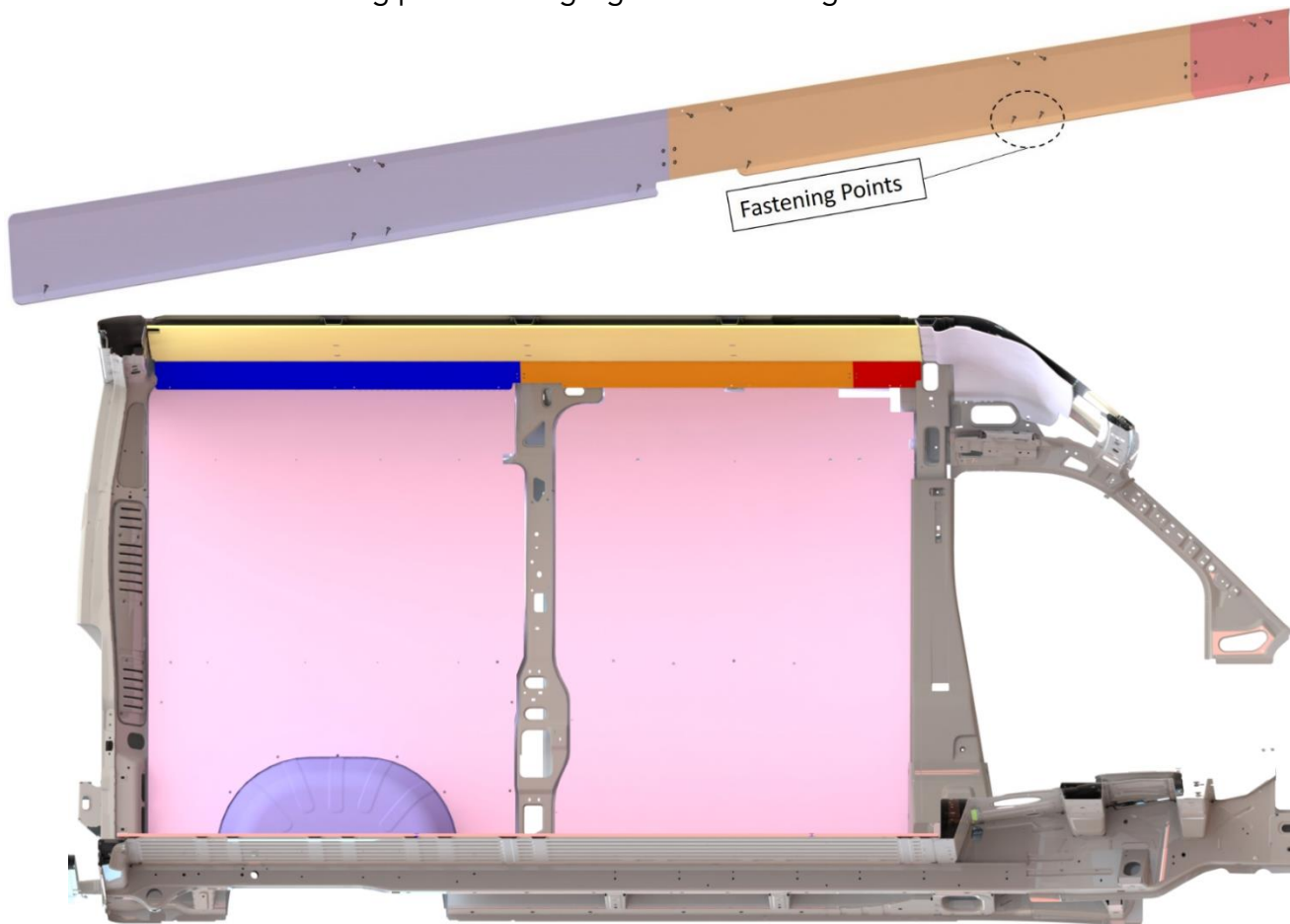
"Driver Side Top Sills Installed" This is view from inside the vehicle when Viewing from Passenger Side
