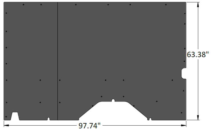
DRIVER SIDE REAR LOWER WALL (D2A)
