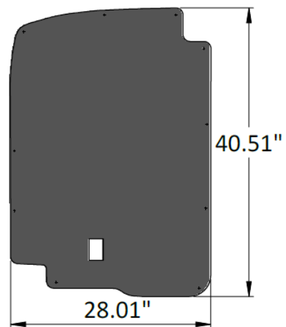
PASSENGER SIDE REAR DOOR LINER (PRA)
